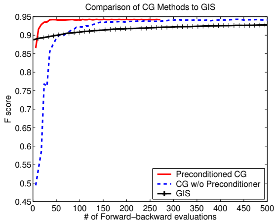
Figure 3: Test F scores vs. training time
