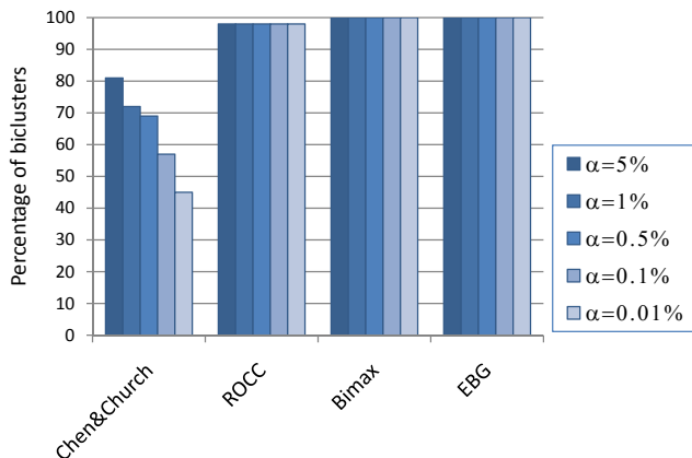
Figure 3: The experimental results on the yeast gene expression data. The y-axis is the percentage of gene clusters that are overrepresented by at least one GO annotation, with five different significance levels ( \alpha ).
