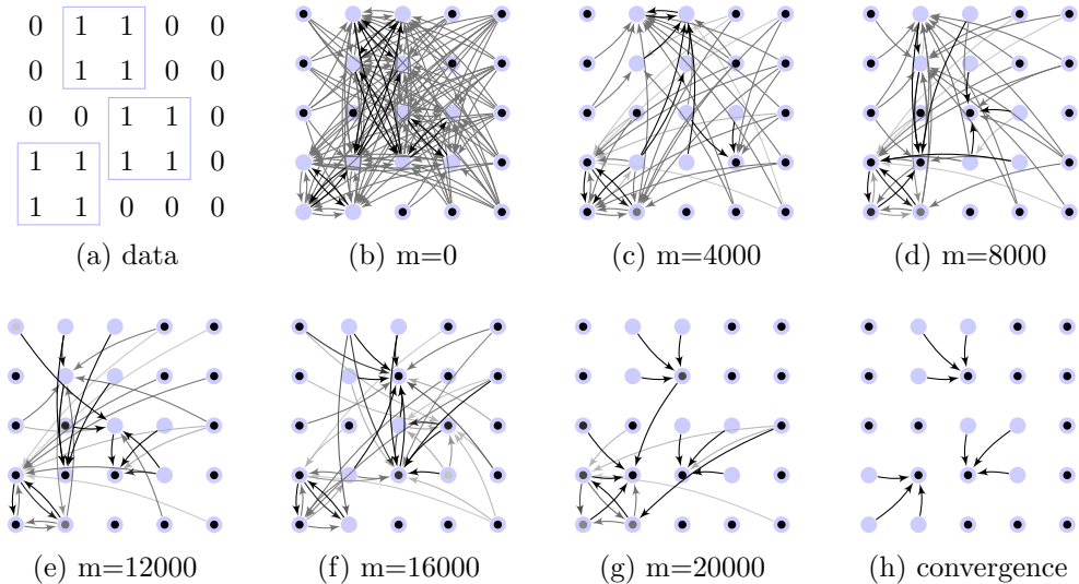
Figure 2: An illustrative example of biclustering using message passing. (a) The data matrix. The best biclustering configuration is denoted by the three boxes. (b)-(h) The exemplar preferences at different stages of the algorithm. m is the number of messages propagated. An edge from node i to node j denotes that node i prefers node j as a candidate exemplar; a dot at node i denotes that node i chooses itself as a candidate exemplar; the grayscale of the edges and dots represents the strength of the preference.
