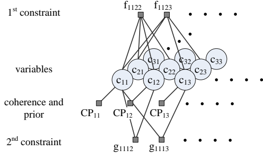
Figure 1: The factor graph representing the factorization of the objective function. Each circle represents a variable. Each box is a factor, connected to the variables it depends on.
